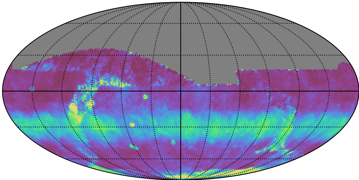
baseline_v3.2_10yrs All sky z band: Median normairmass
