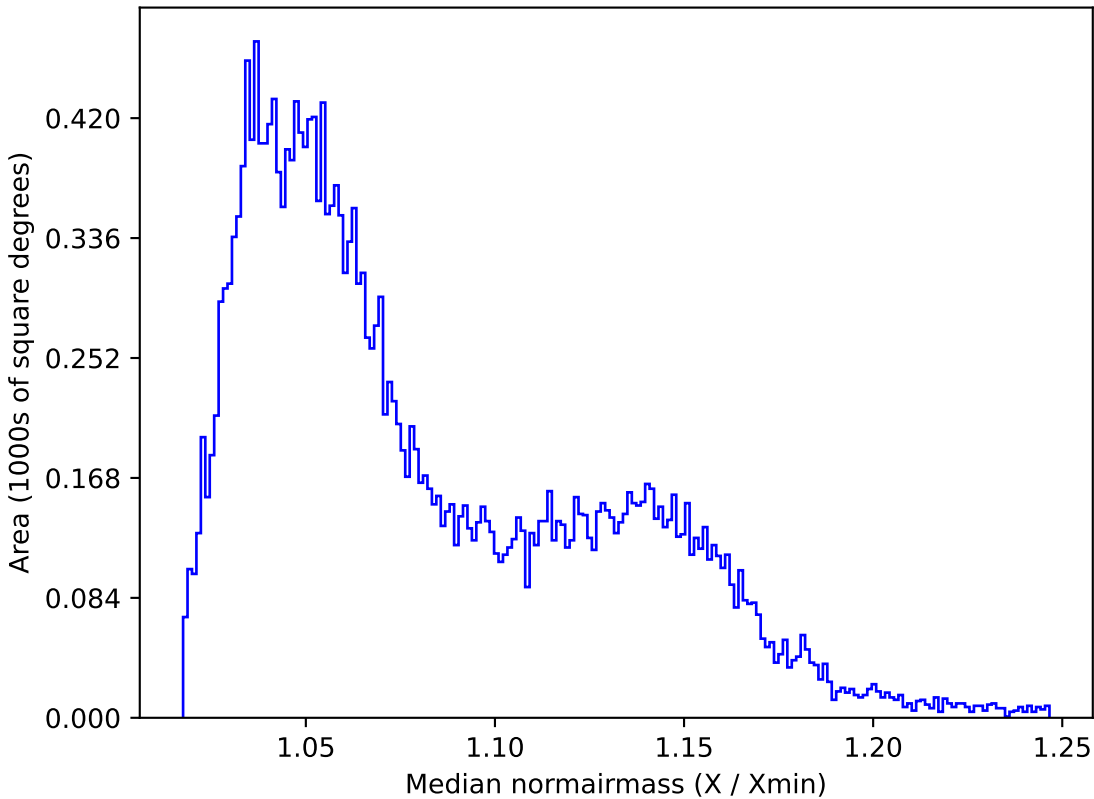
baseline_v3.2_10yrs All sky z band: Median normairmass
