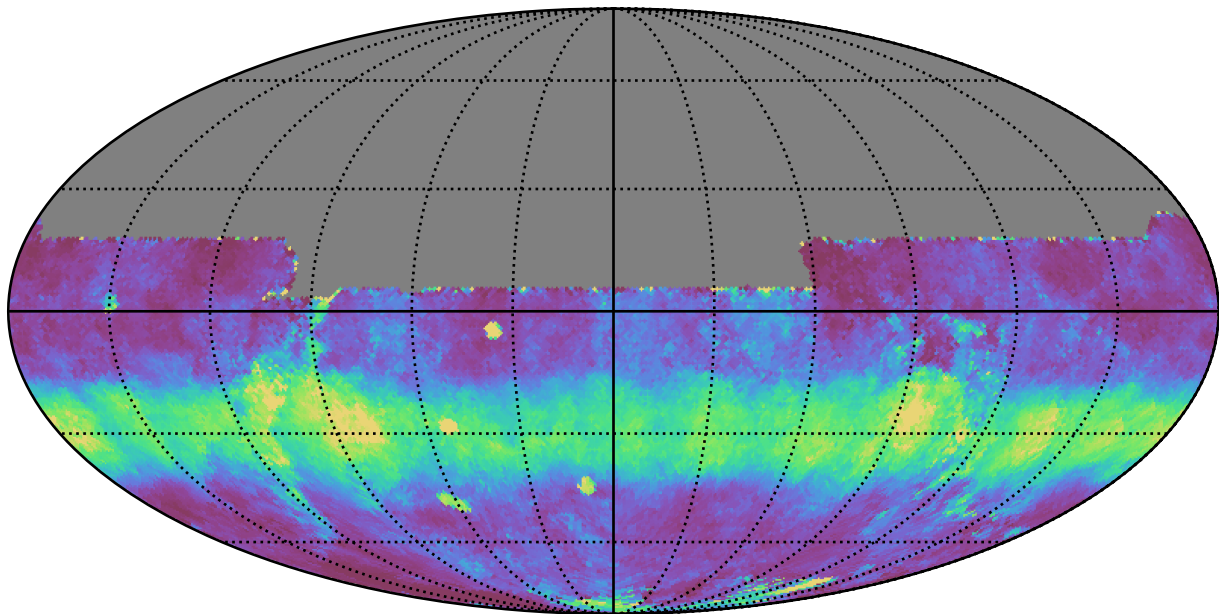
baseline_v3.2_10yrs All sky y band: Median normairmass
