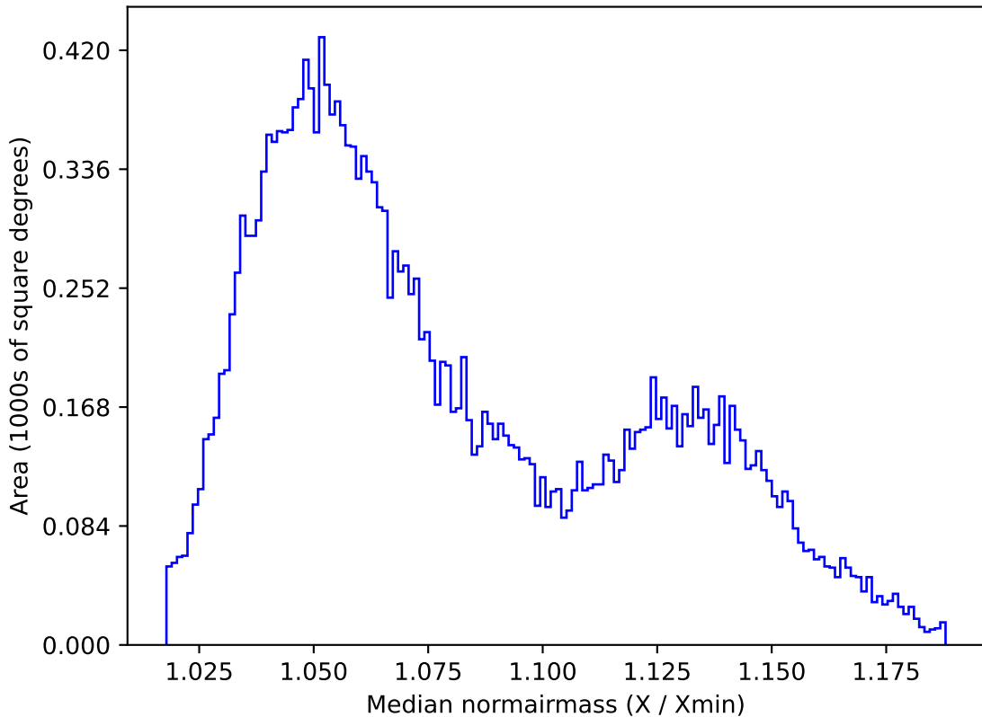
baseline_v3.2_10yrs All sky y band: Median normairmass
