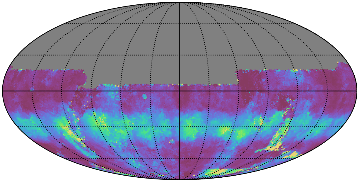
baseline_v3.2_10yrs All sky u band: Median normairmass
