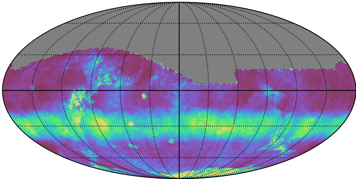
baseline_v3.2_10yrs All sky r band: Median normairmass
