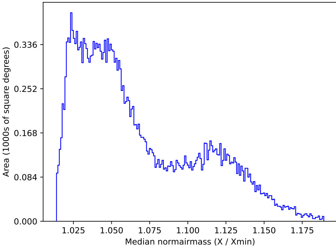
baseline_v3.2_10yrs All sky r band: Median normairmass
