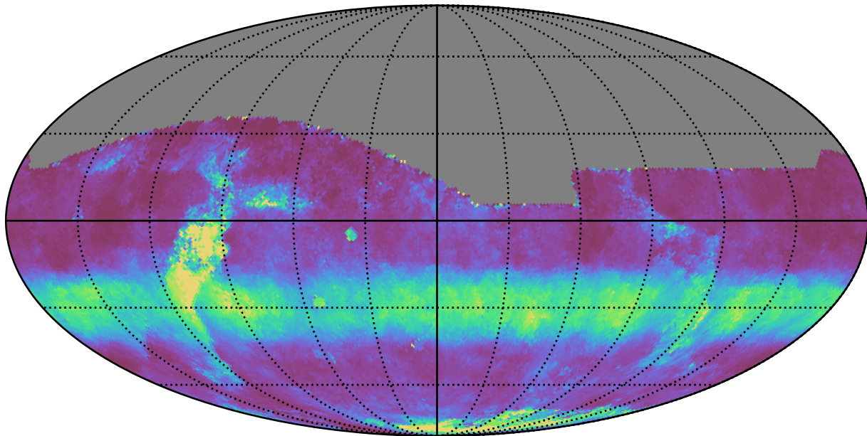
baseline_v3.2_10yrs All sky i band: Median normairmass
