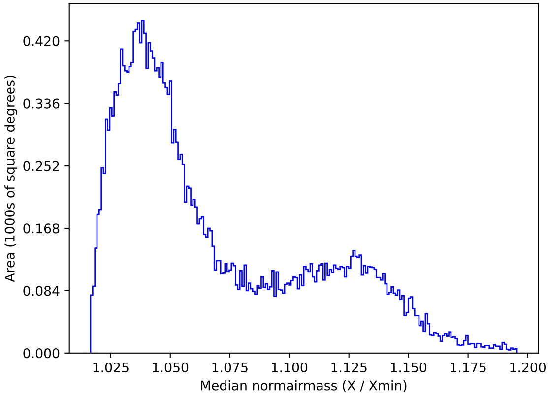
baseline_v3.2_10yrs All sky i band: Median normairmass
