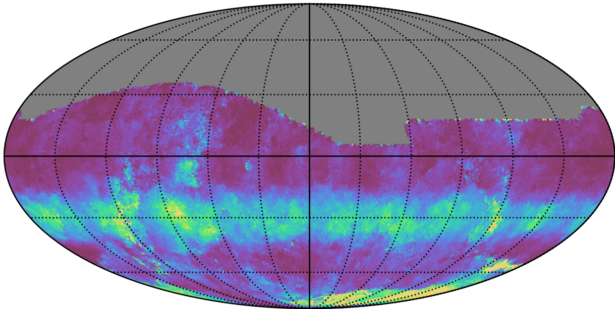
baseline_v3.2_10yrs All sky g band: Median normairmass
