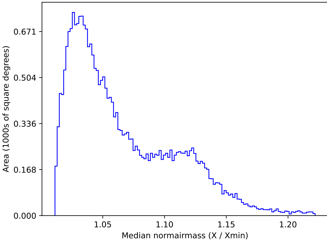
baseline_v3.2_10yrs All sky g band: Median normairmass
