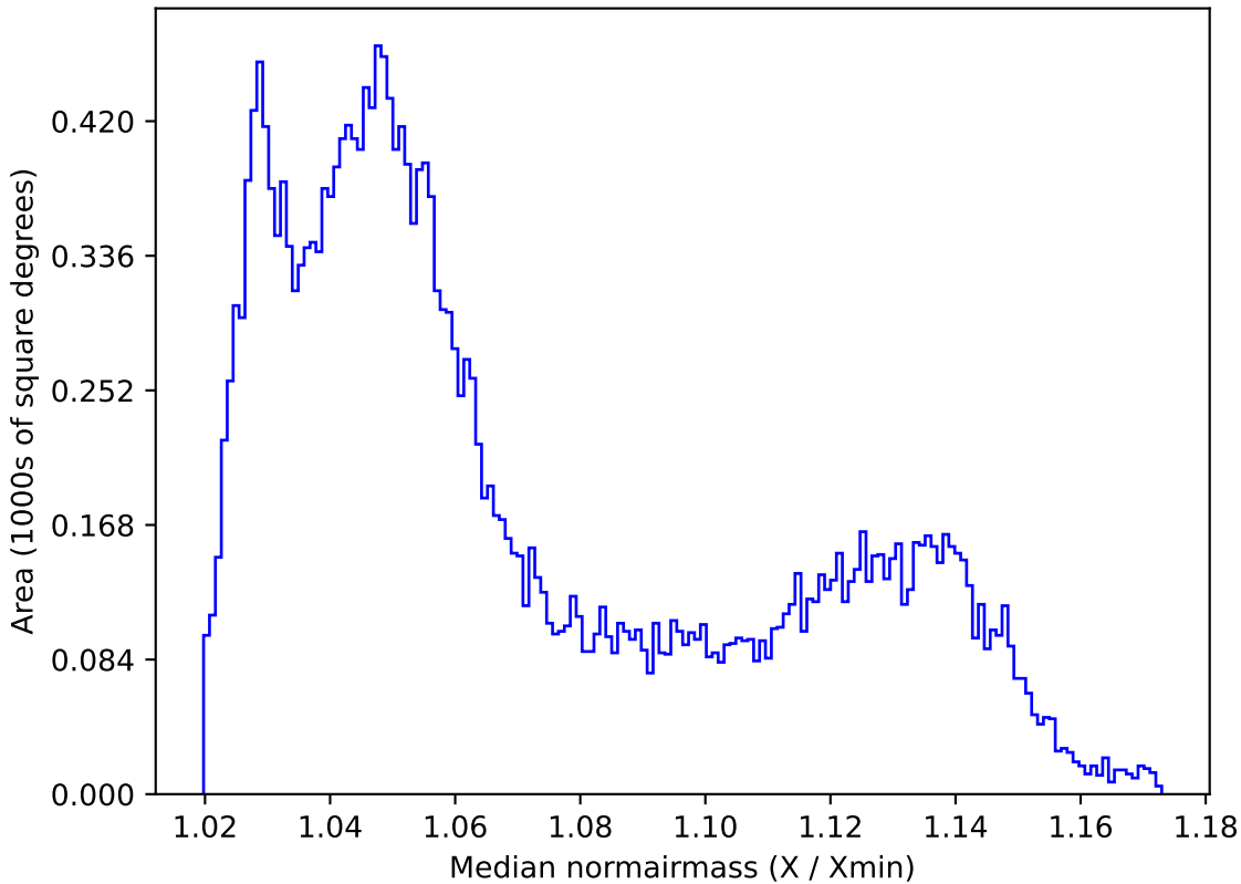
baseline_v3.2_10yrs All sky all bands: Median normairmass
