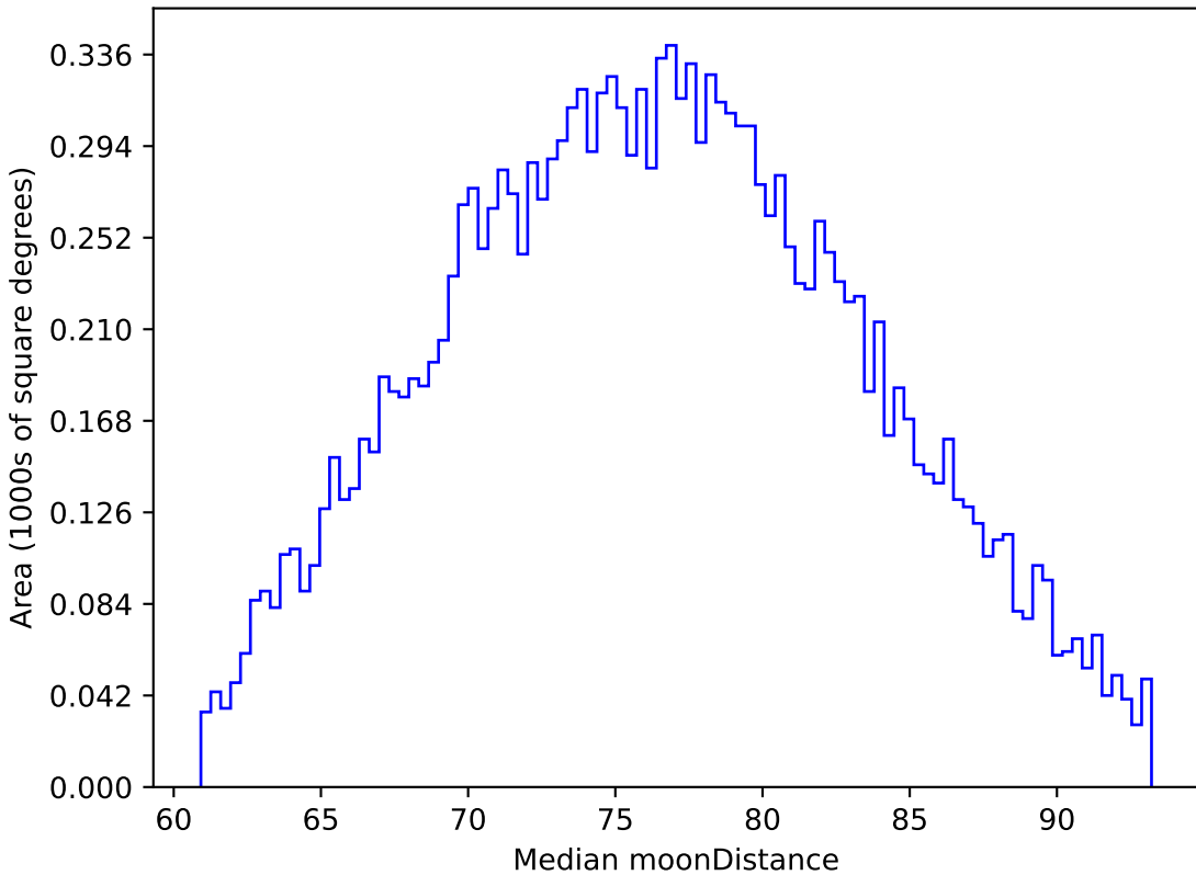
baseline_v3.2_10yrs WFD z band: Median moonDistance
