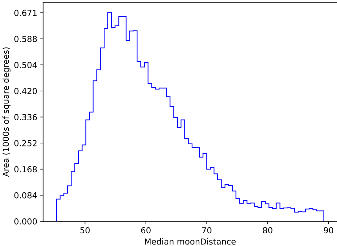
baseline_v3.2_10yrs WFD y band: Median moonDistance
