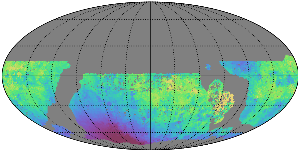
baseline_v3.2_10yrs WFD u band: Median moonDistance
