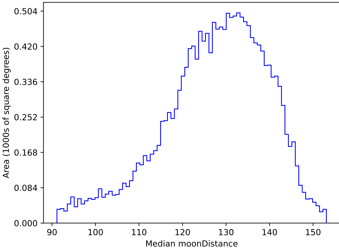
baseline_v3.2_10yrs WFD u band: Median moonDistance
