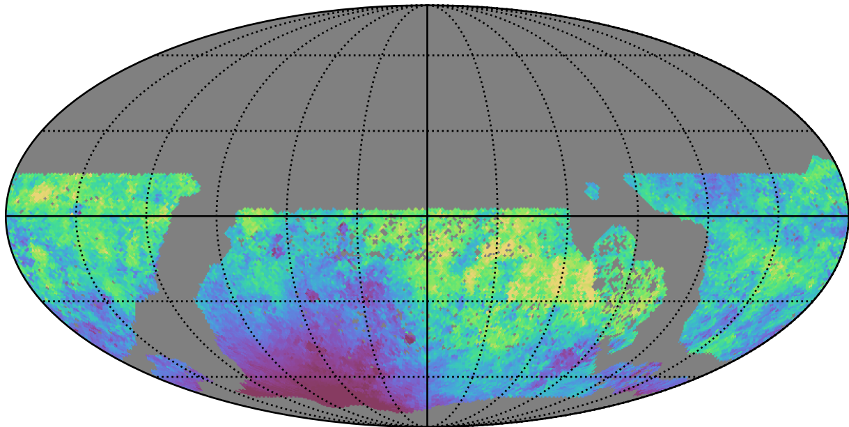
baseline_v3.2_10yrs WFD r band: Median moonDistance
