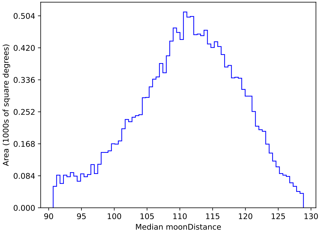
baseline_v3.2_10yrs WFD r band: Median moonDistance
