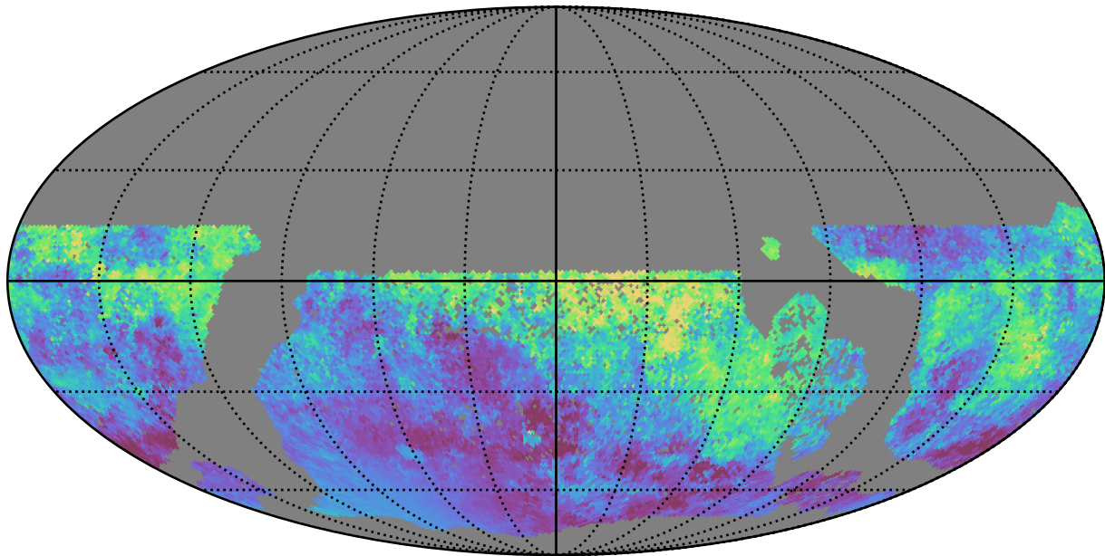
baseline_v3.2_10yrs WFD i band: Median moonDistance
