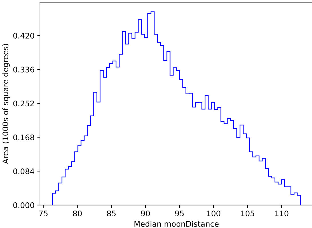
baseline_v3.2_10yrs WFD i band: Median moonDistance
