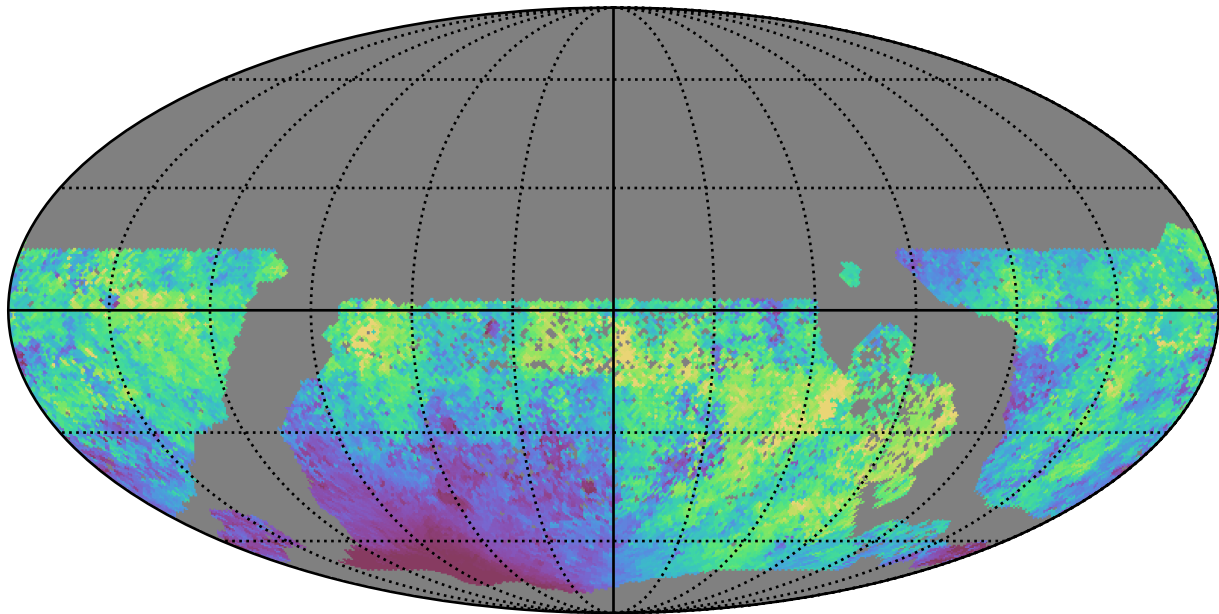
baseline_v3.2_10yrs WFD g band: Median moonDistance
