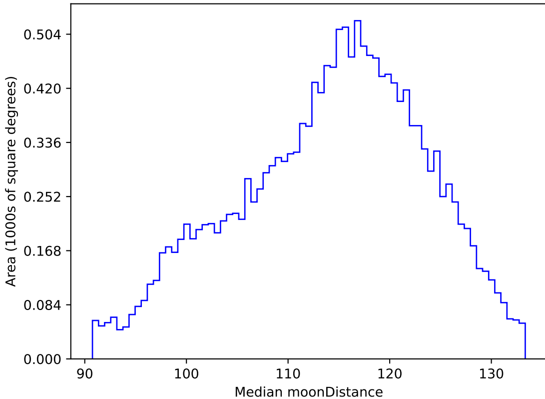
baseline_v3.2_10yrs WFD g band: Median moonDistance
