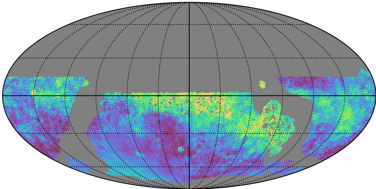
baseline_v3.2_10yrs WFD all bands: Median moonDistance
