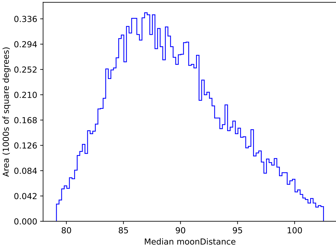
baseline_v3.2_10yrs WFD all bands: Median moonDistance
