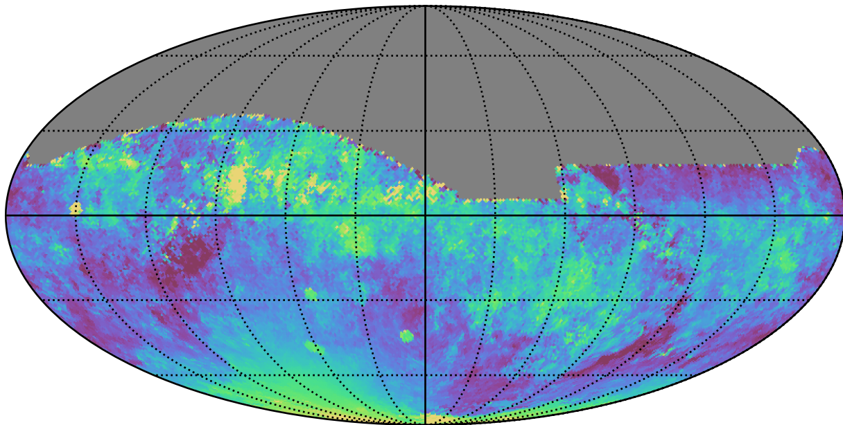
baseline_v3.2_10yrs All sky z band: Median moonDistance
