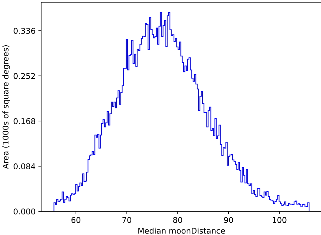
baseline_v3.2_10yrs All sky z band: Median moonDistance
