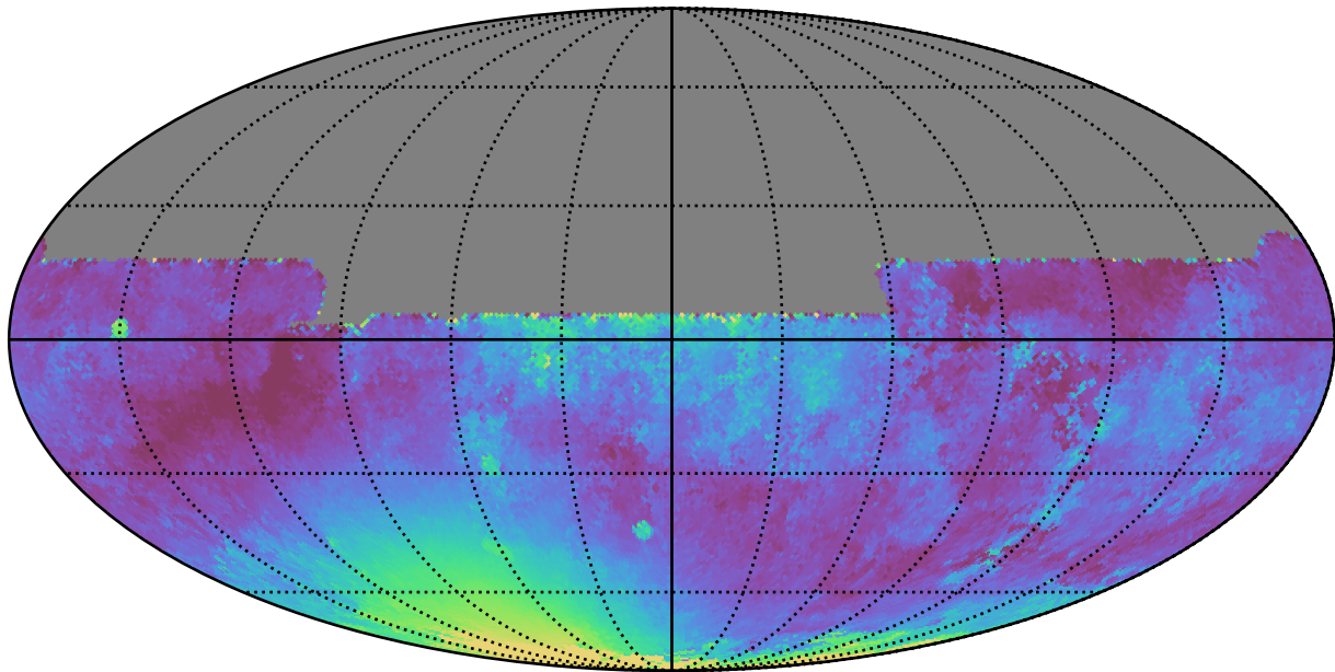
baseline_v3.2_10yrs All sky y band: Median moonDistance
