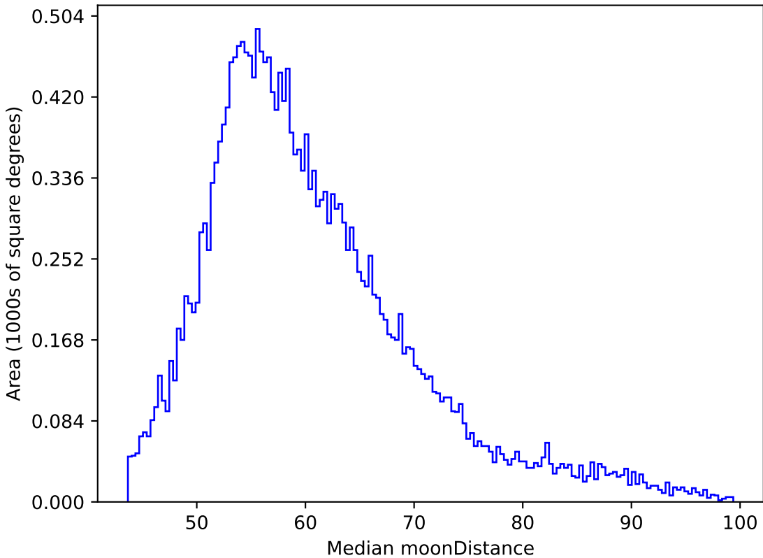
baseline_v3.2_10yrs All sky y band: Median moonDistance
