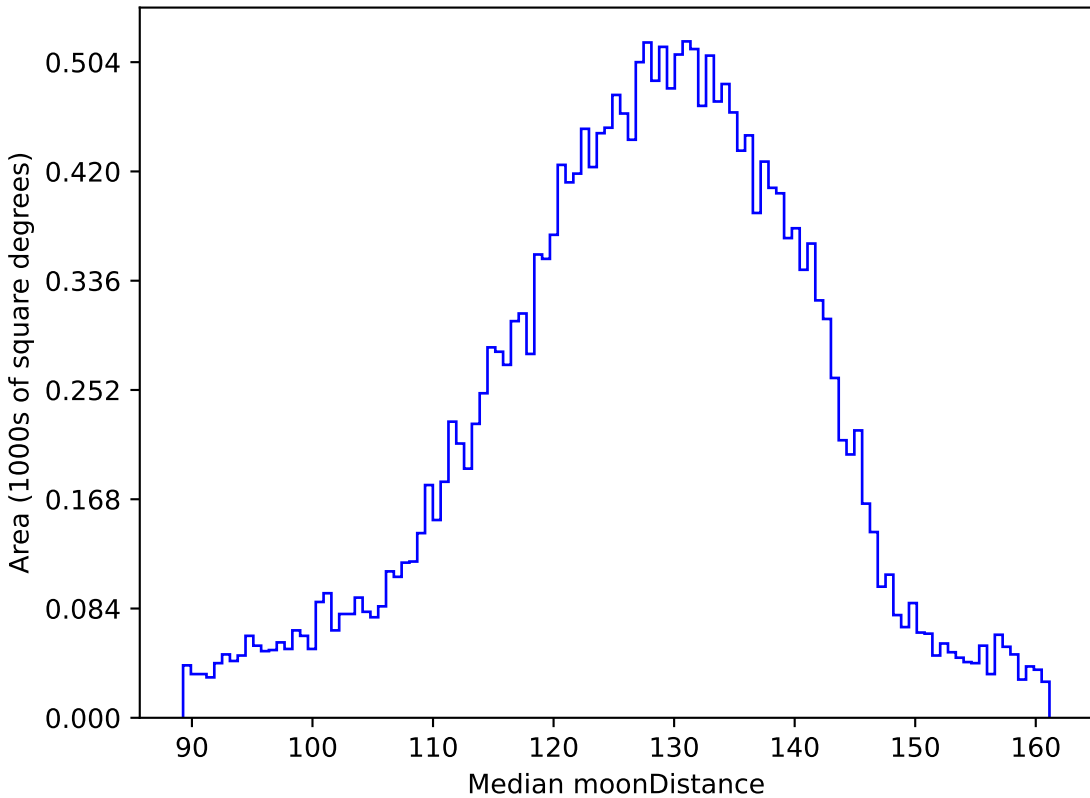
baseline_v3.2_10yrs All sky u band: Median moonDistance
