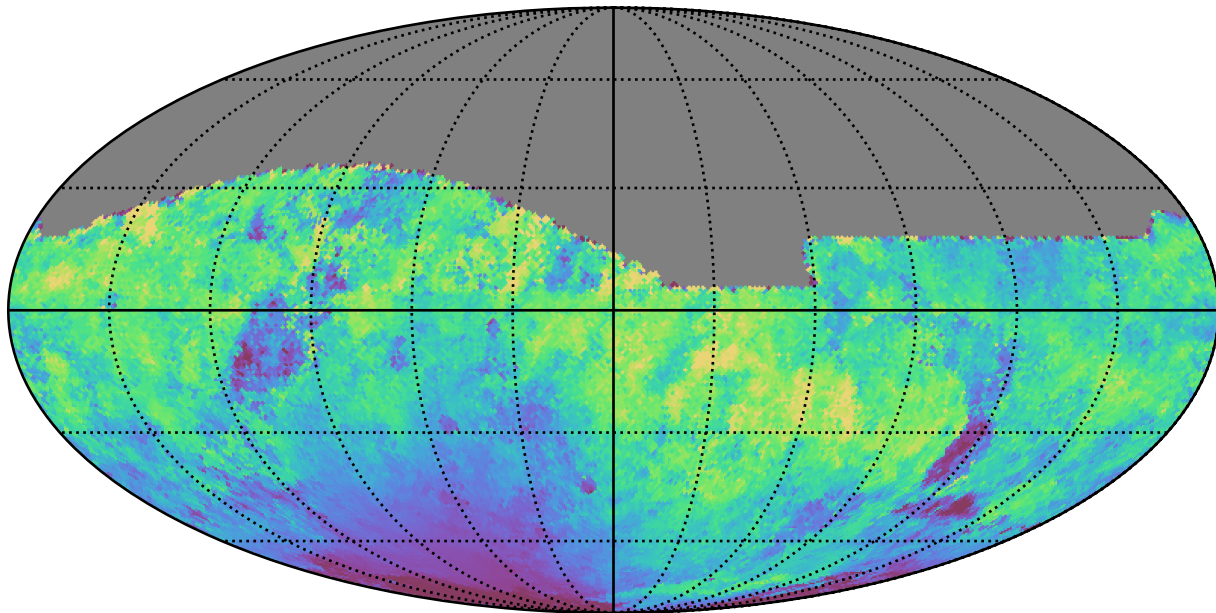
baseline_v3.2_10yrs All sky r band: Median moonDistance
