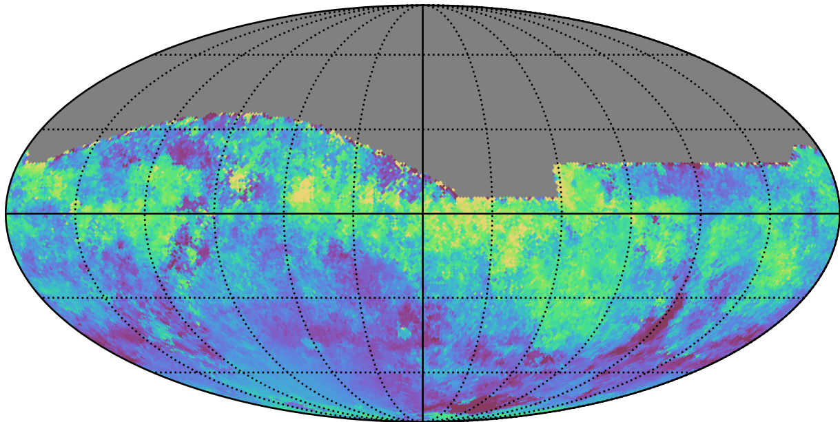
baseline_v3.2_10yrs All sky i band: Median moonDistance
