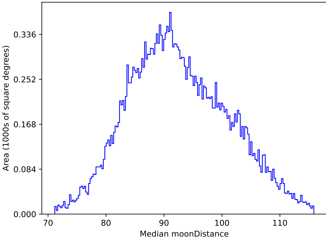
baseline_v3.2_10yrs All sky i band: Median moonDistance
