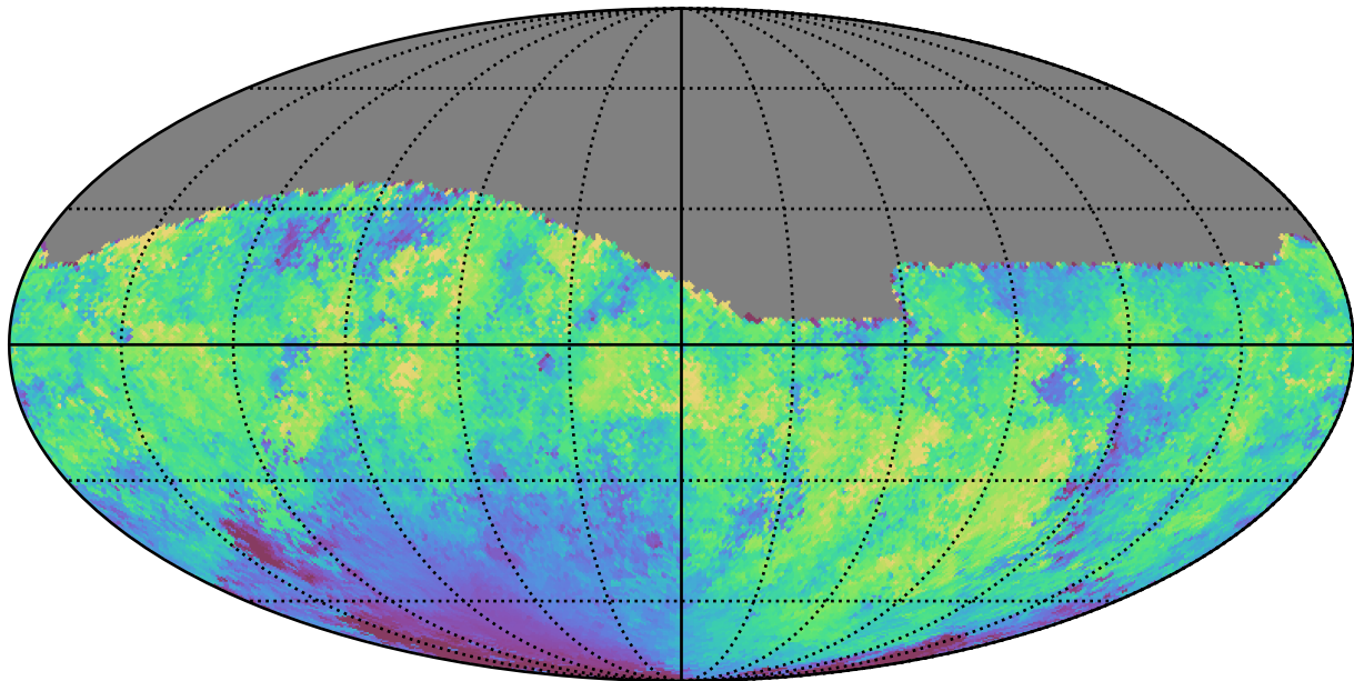
baseline_v3.2_10yrs All sky g band: Median moonDistance
