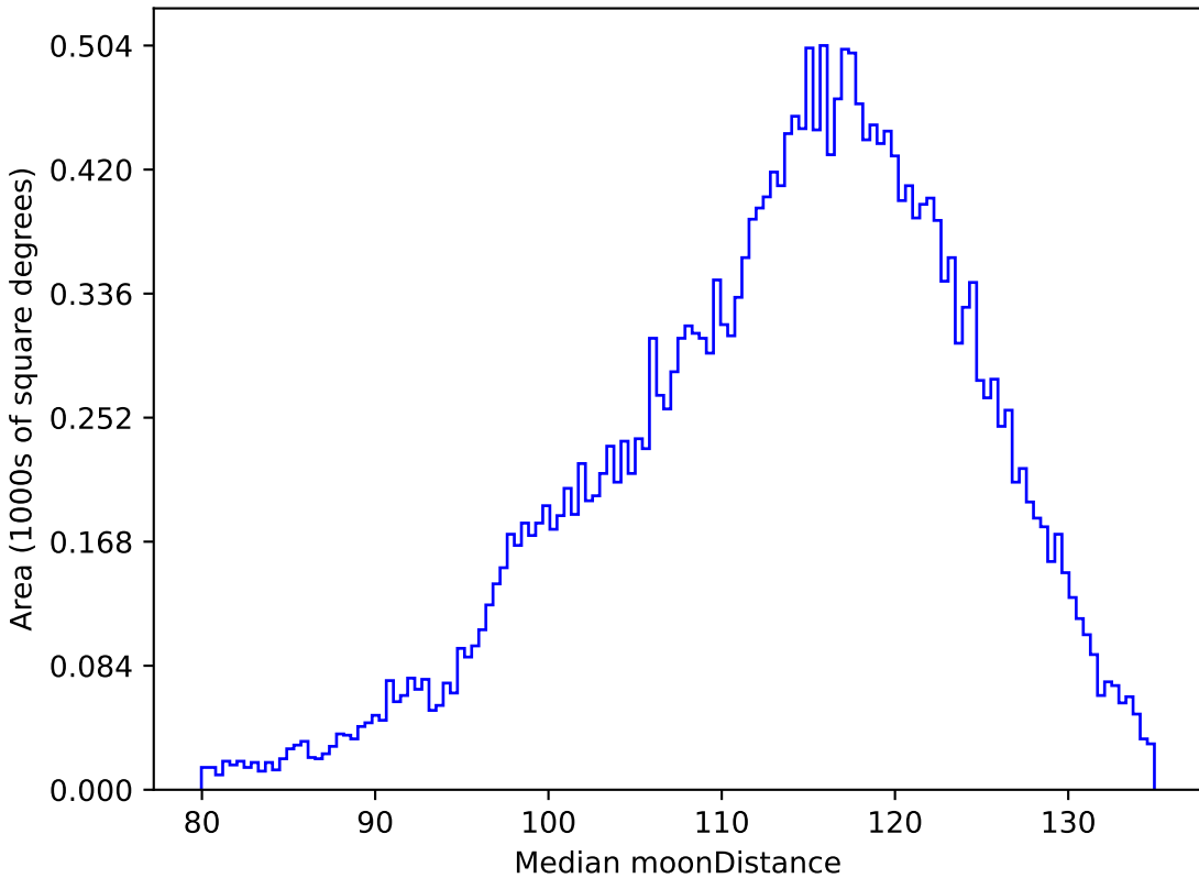
baseline_v3.2_10yrs All sky g band: Median moonDistance
