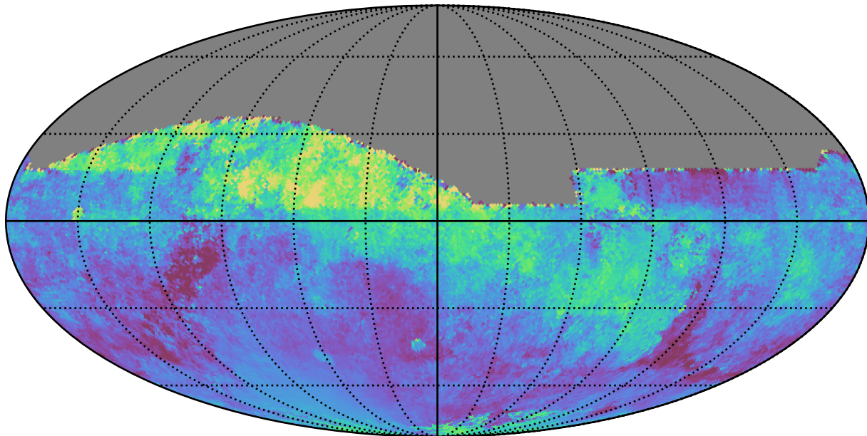
baseline_v3.2_10yrs All sky all bands: Median moonDistance
