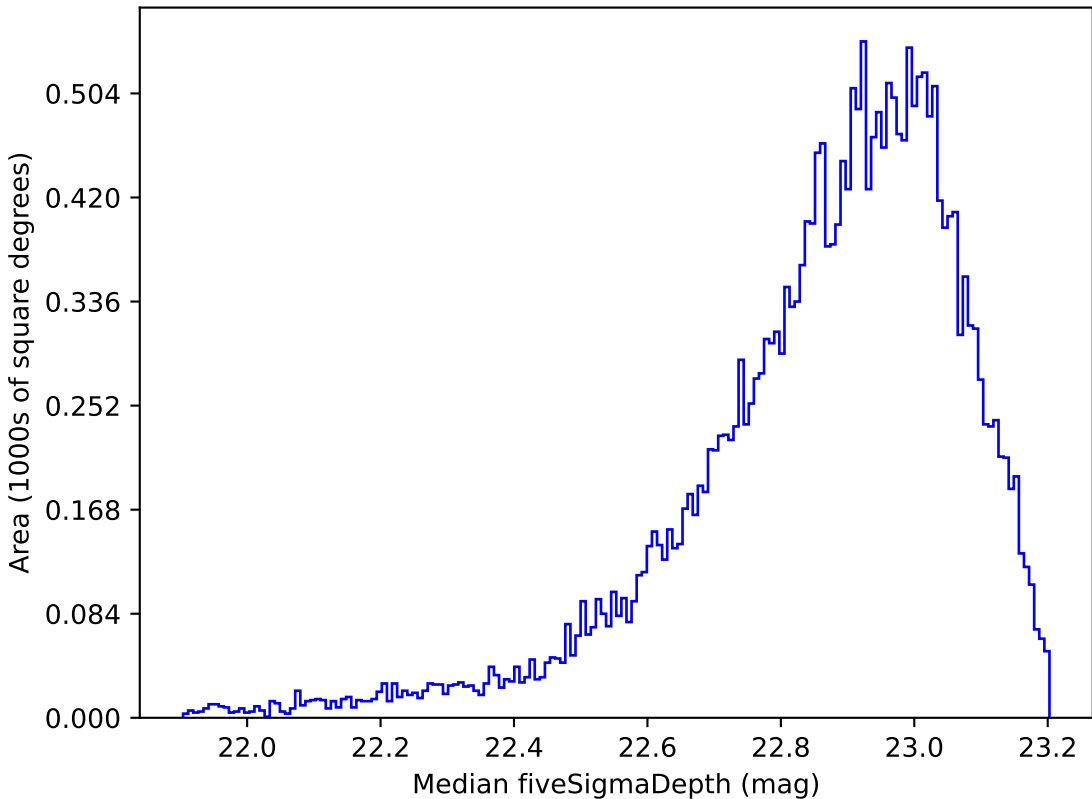
baseline_v3.2_10yrs Yr 1 z band: Median fiveSigmaDepth
