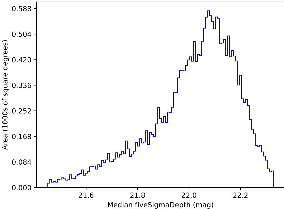
baseline_v3.2_10yrs Yr 1 y band: Median fiveSigmaDepth
