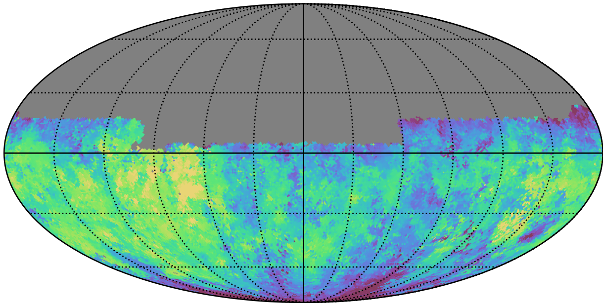
baseline_v3.2_10yrs Yr 1 u band: Median fiveSigmaDepth
