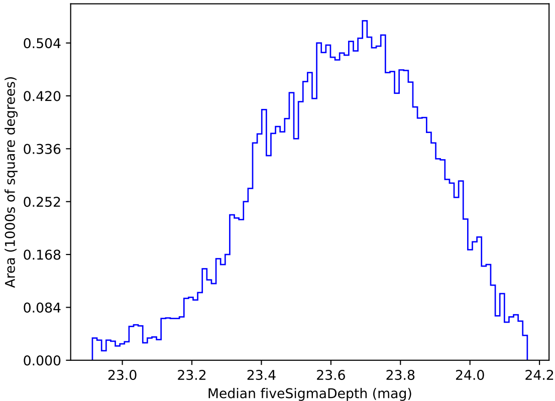
baseline_v3.2_10yrs Yr 1 u band: Median fiveSigmaDepth
