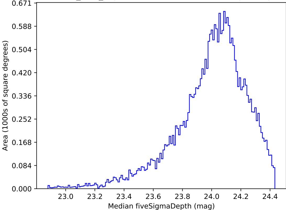
baseline_v3.2_10yrs Yr 1 r band: Median fiveSigmaDepth
