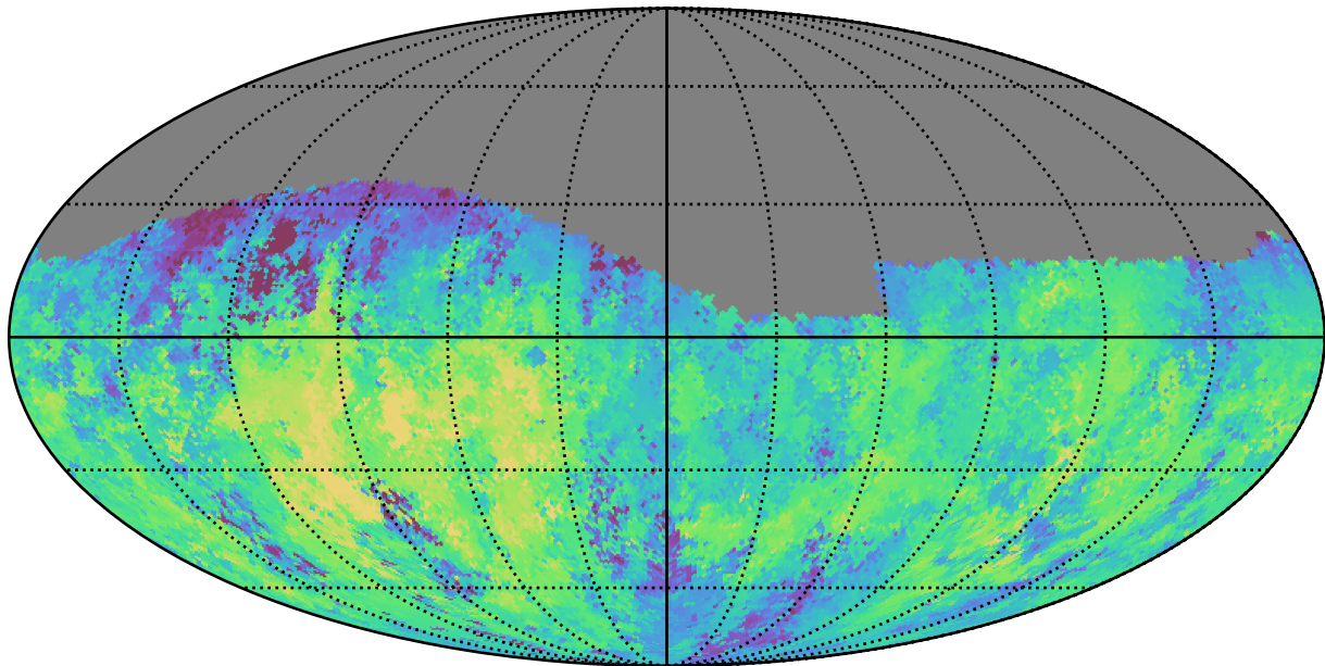
baseline_v3.2_10yrs Yr 1 g band: Median fiveSigmaDepth
