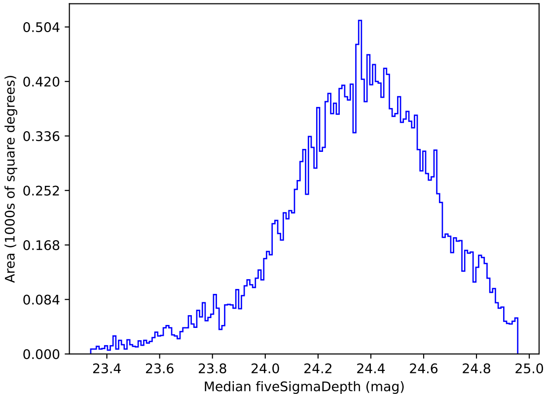
baseline_v3.2_10yrs Yr 1 g band: Median fiveSigmaDepth
