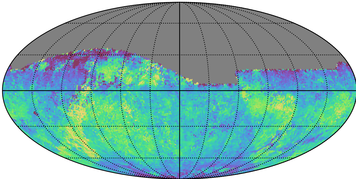
baseline_v3.2_10yrs Yr 1 all bands: Median fiveSigmaDepth
