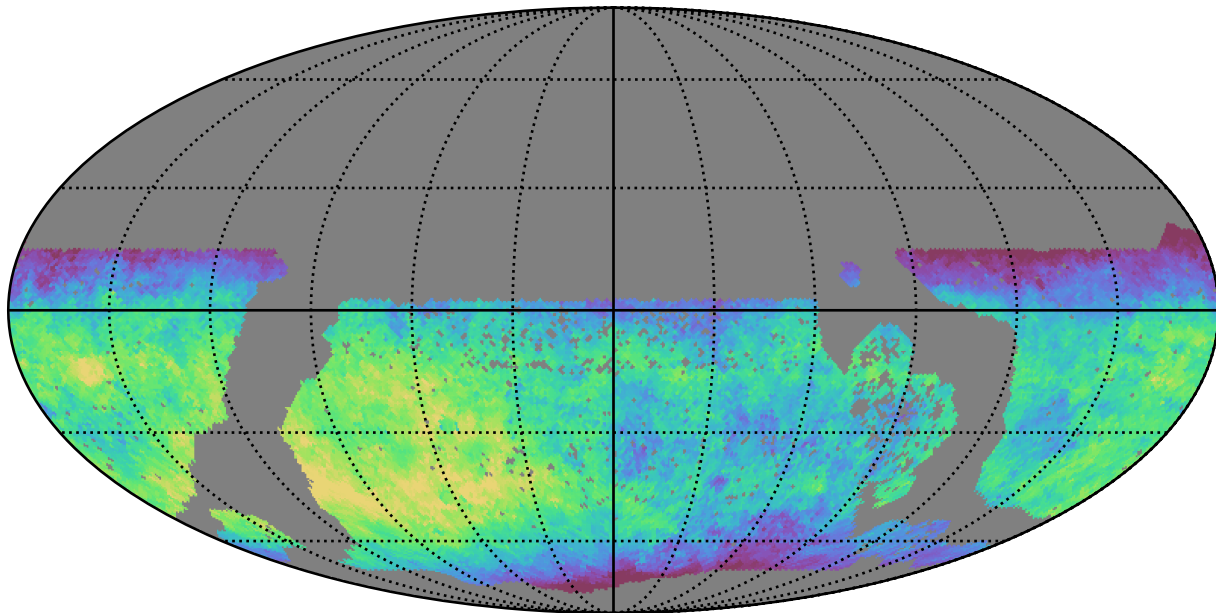
baseline_v3.2_10yrs WFD z band: Median fiveSigmaDepth
