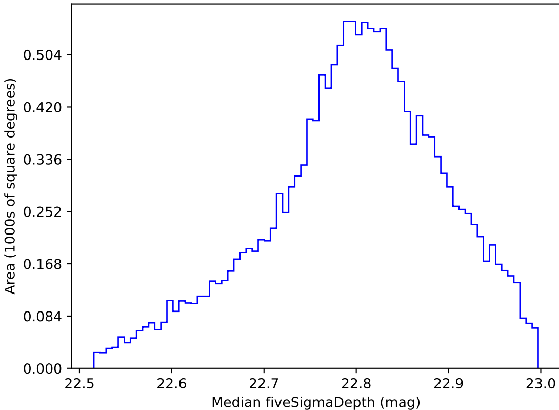
baseline_v3.2_10yrs WFD z band: Median fiveSigmaDepth
