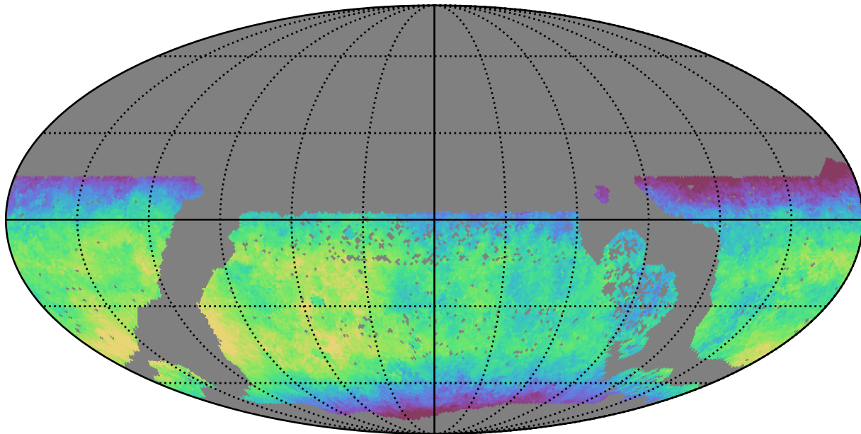
baseline_v3.2_10yrs WFD y band: Median fiveSigmaDepth
