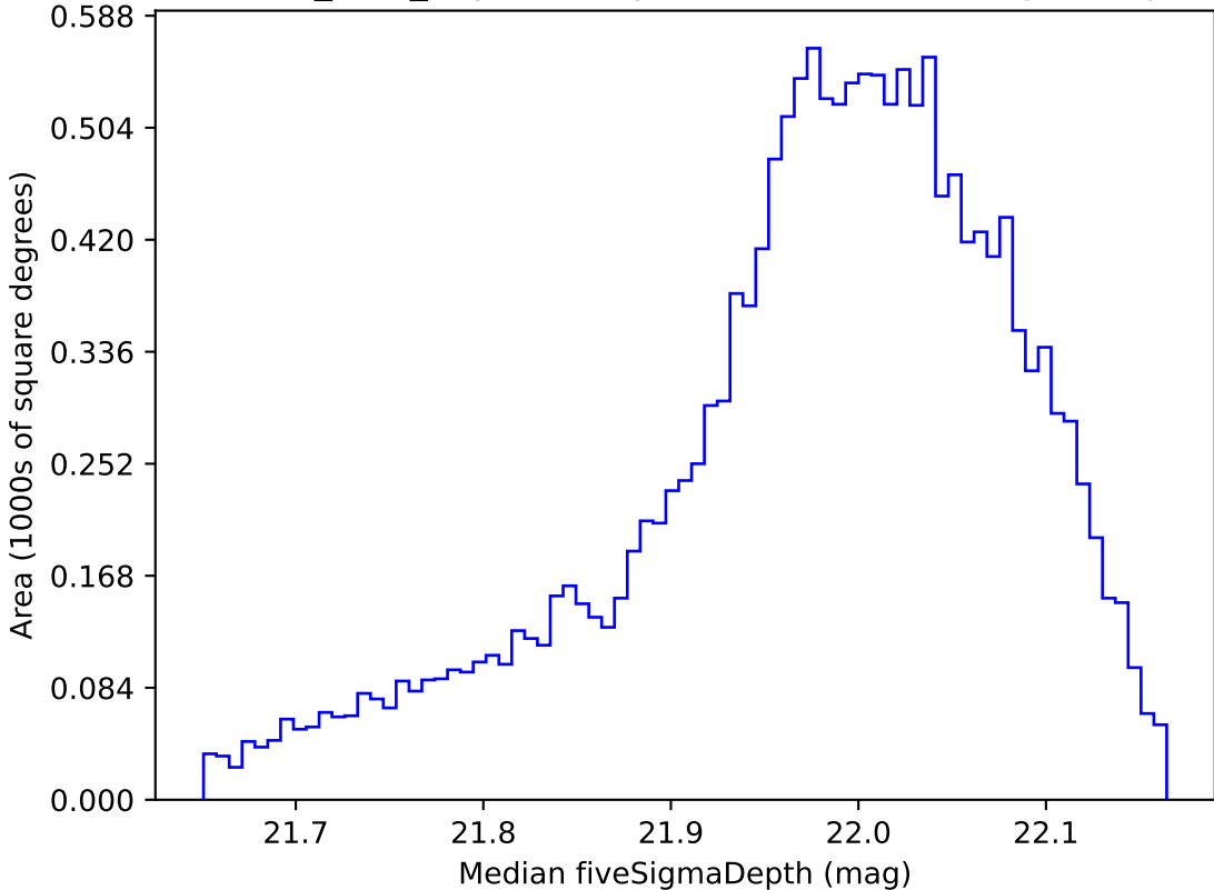
baseline_v3.2_10yrs WFD y band: Median fiveSigmaDepth
