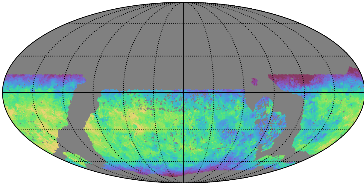
baseline_v3.2_10yrs WFD u band: Median fiveSigmaDepth
