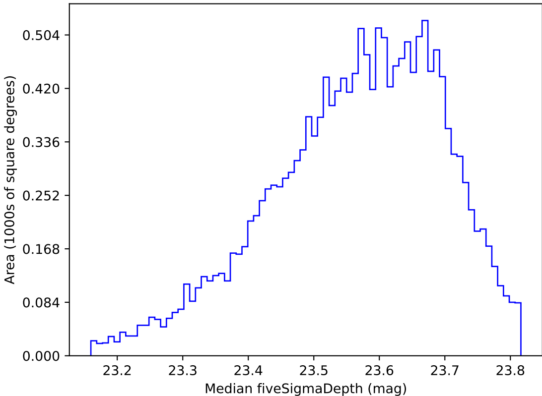
baseline_v3.2_10yrs WFD u band: Median fiveSigmaDepth
