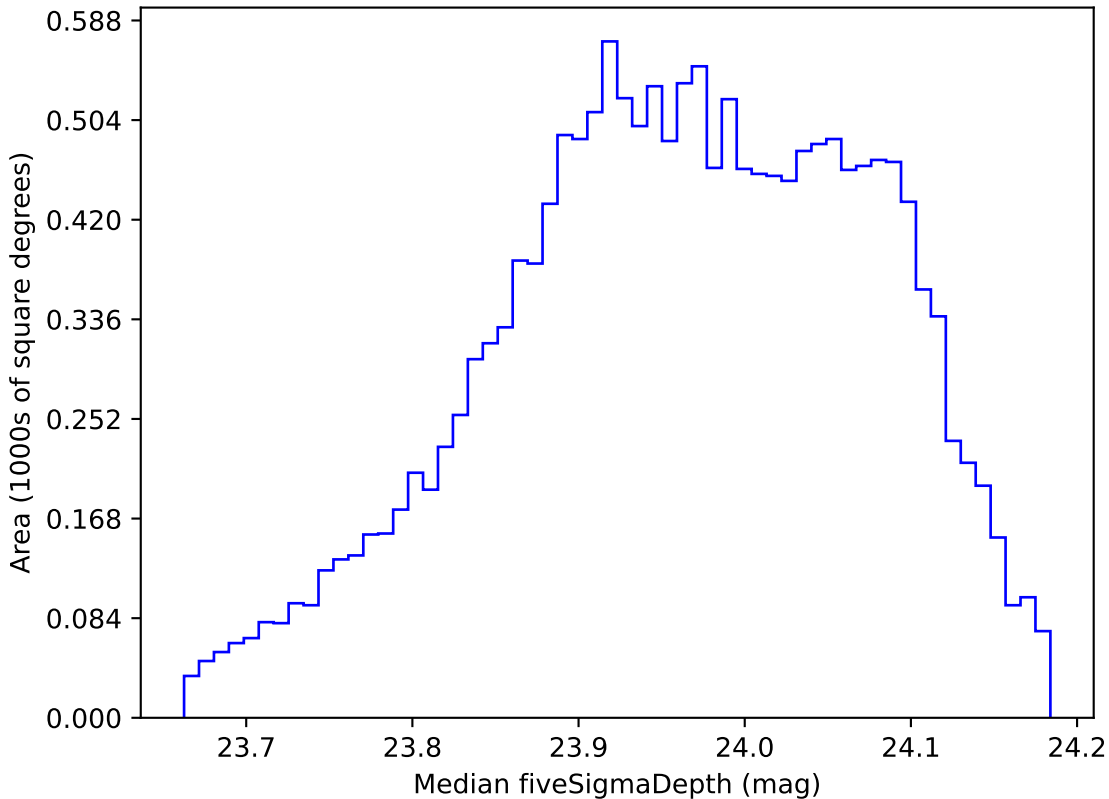
baseline_v3.2_10yrs WFD r band: Median fiveSigmaDepth
